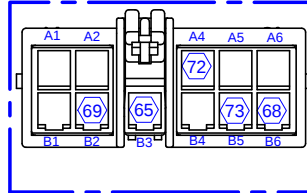
VIEW C TYCO 144521-4 CONTACT 144180-1
