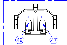
VIEW F DELPHI 12010973 CONTACT 12124582 SEAL 15324982
