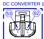
VIEW B DELPHI 12015792 CONTACT 12124580 SEAL 15324982
