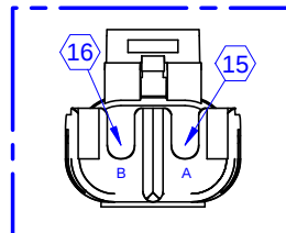
VIEW J DELPHI 12015792 CONTACT 12089188 SEAL 15324982
