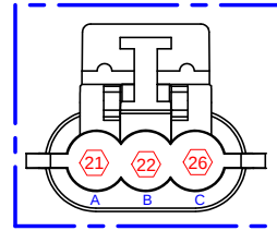
VIEW L DELPHI 12110293 CONTACT 12048074
