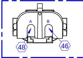
VIEW E DELPHI 12010973 CONTACT 12124582
