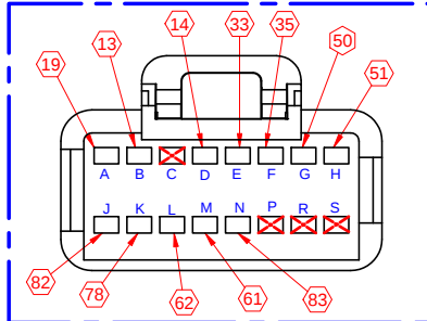
VIEW I DELPHI 15332177 CONTACT 12191812
