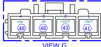
VIEW G MOLEX 42816-0412 CONTACT 42815-0011
