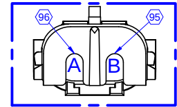
VIEW D DELPHI 12010973 CONTACT 12089040 SEAL 15324982
