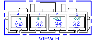
VIEW H MOLEX 42816-0412 CONTACT 42815-0011
