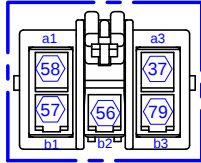
VIEW A TYCO 144518-1 CONTACT 144180-1
