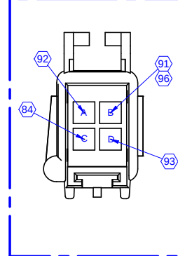
VIEW U DELPHI 12129135 PIN 12020116 LOCK 12129137
