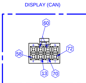
VIEW J MOLEX 39-01-2080 PLUG CONTACT 39-00-0039
