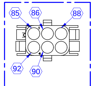
VIEW V AMP 1-480705-0 PIN 350218-1 WIRE SEAL 794276-1 SEALING PLUG 770377-1
