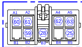
VIEW B TYCO 144520-2 CONTACT 144180-1
