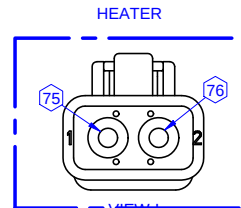
VIEW L DEUTSCH DTP06-2S CONTACT 1062-12-0222 WEDGE LOCK WP-2S
