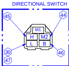
VIEW F DELPHI 2973422 CONTACT 12124512 (CIRCUITS 30 & 47 12124520)
