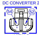
VIEW C DELPHI 12015792 CONTACT 12124580 SEAL 15324982
