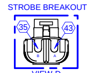
VIEW D DELPHI 12015792 CONTACT 12089188 SEAL 15324982
