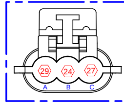
VIEW K DELPHI 12110293 CONTACT 12048074
