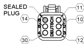
REAR VIEW FOR PAD
