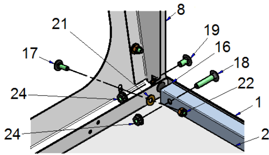
UNDERNEATH VIEW OF TOP FRONT LEFT-HAND CORNER
