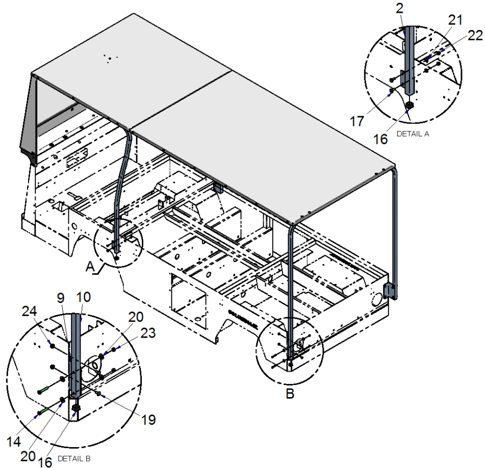
UNDERNEATH VIEW OF TOP MID LEFT-HAND CORNERS
