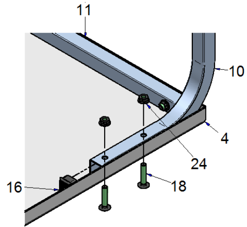
UNDERNEATH VIEW OF TOP REAR LEFT-HAND CORNER
