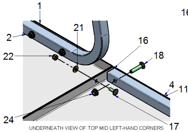
UNDERNEATH VIEW OF TOP MID LEFT-HAND CORNERS
