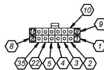
REAR VIEW OF POWER SWITCH CONNECTOR
